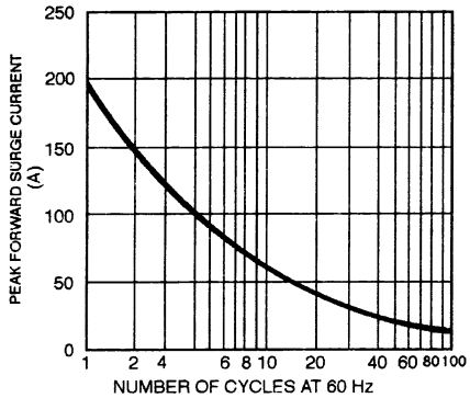
FIG. 1 - MAXIMUM NON-REPETITIVE FORWARD SURGE CURRENT - PER ELEMNET
