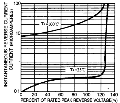
FIG. 4 - TYPICAL REVERSE CHARACTERISTICS PER ELEMNET
