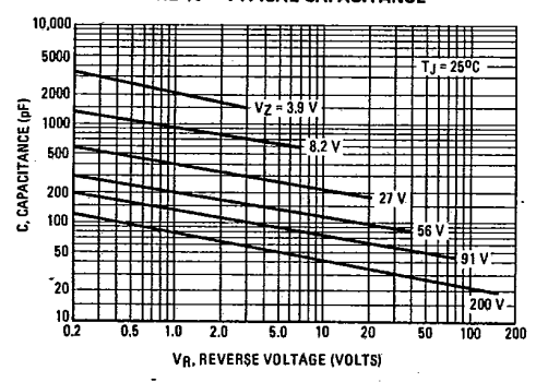
FIGURE 10 - TYPICAL CAPACITANCE
