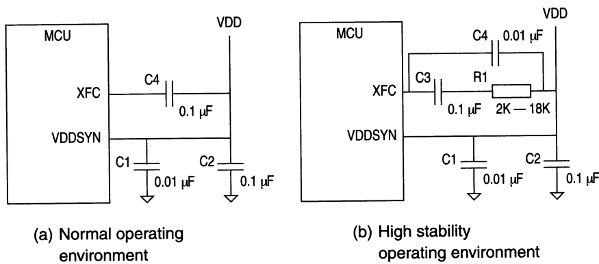
Figure 11-4 System clock filter networks
