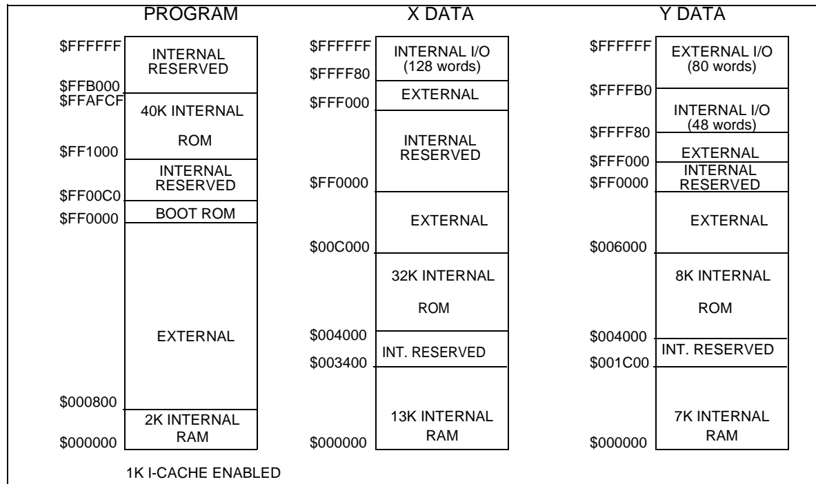
Figure 5-2 Memory Maps for MSW=(X,X), CE=1, MS=0, SC=0
