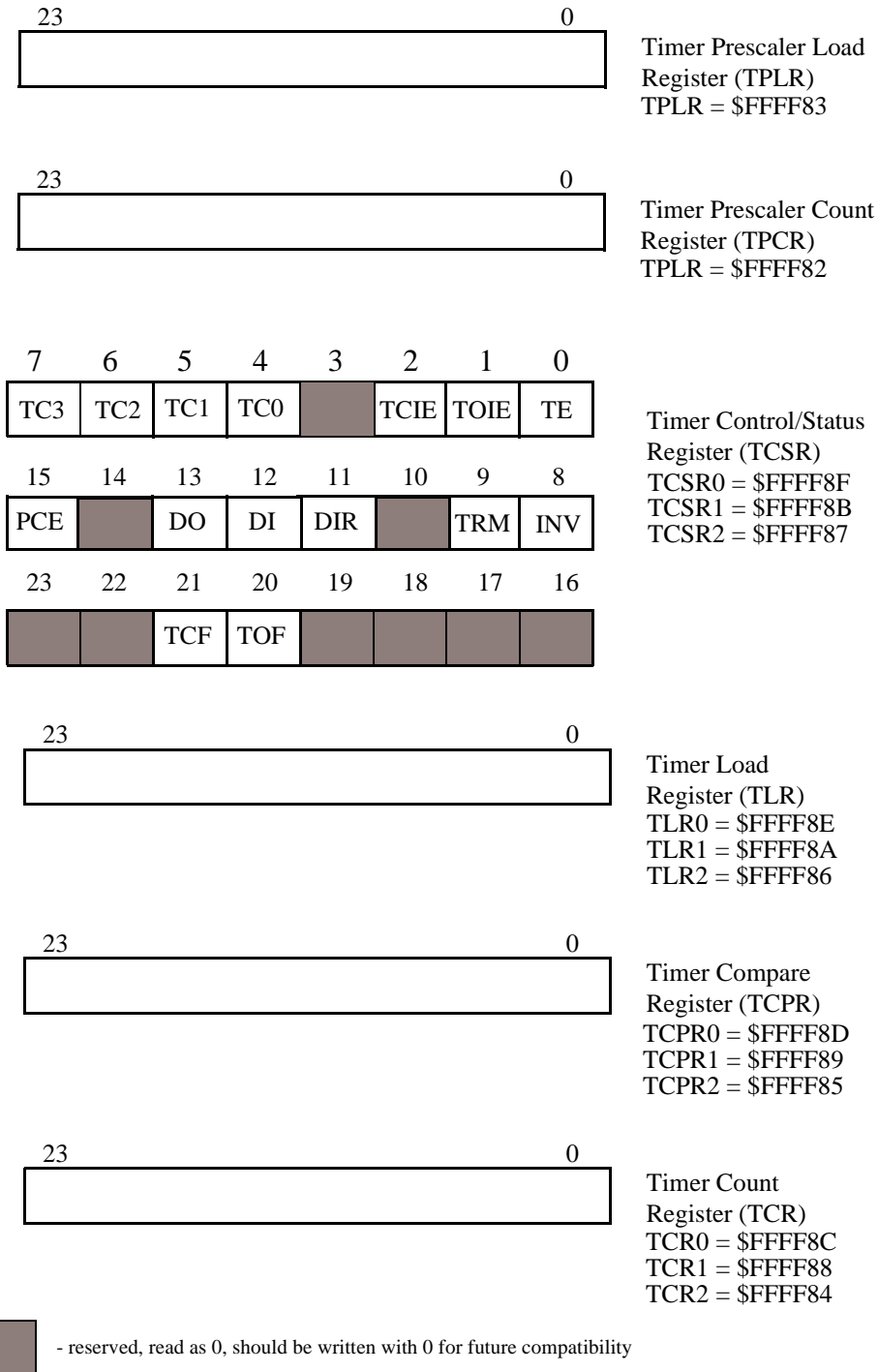
Figure 13-3 Timer Module Programmer's Model
