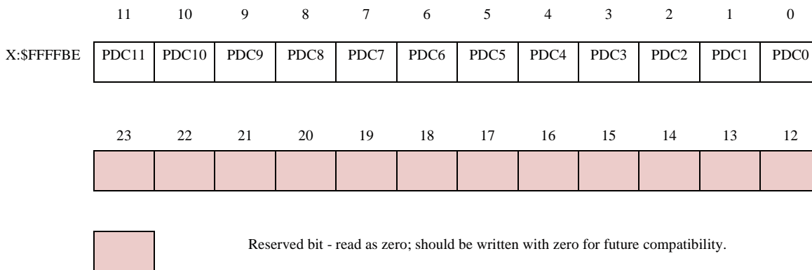
Figure 10-20 PRRC Register
