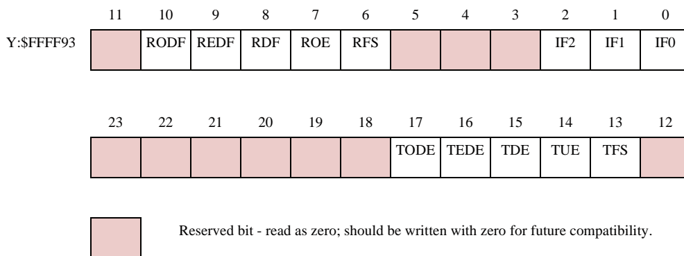
Figure 11-10 SAISR_1 Register
