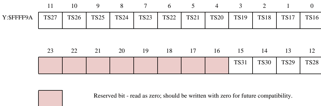
Figure 11-12 TSMB_1 Register
