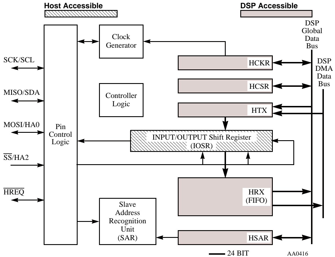
Figure 9-1 Serial Host Interface Block Diagram
