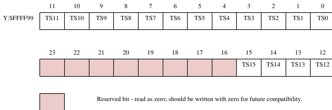
Figure 11-11 TSMA_1 Register
