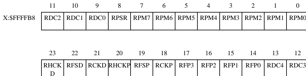
Figure 10-8 RCCR Register
