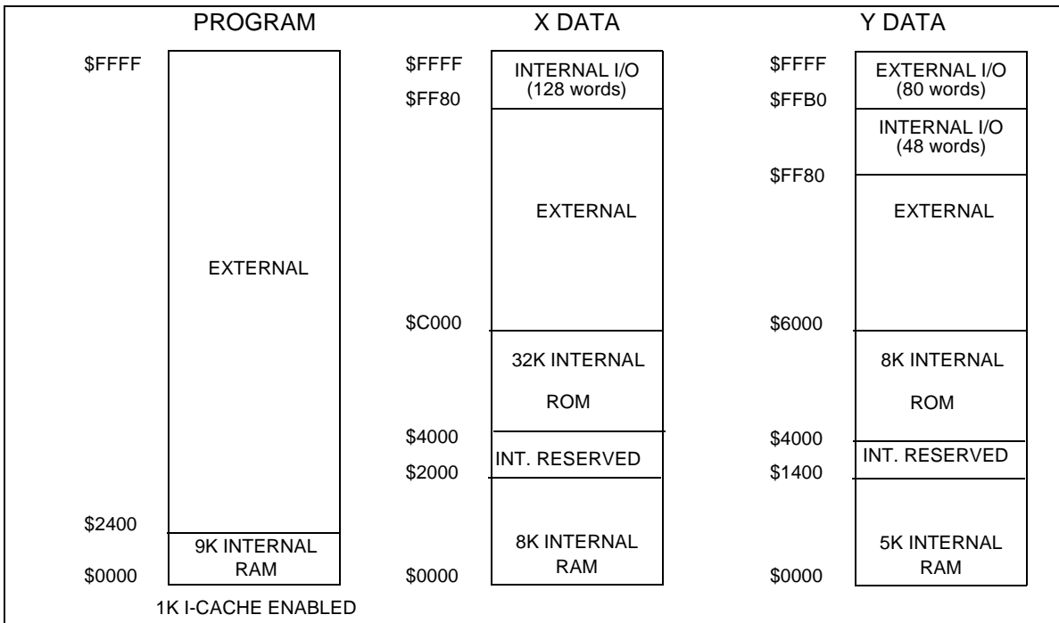
Figure 5-14 Memory Maps for MSW=(0,0), CE=1, MS=1, SC=1
