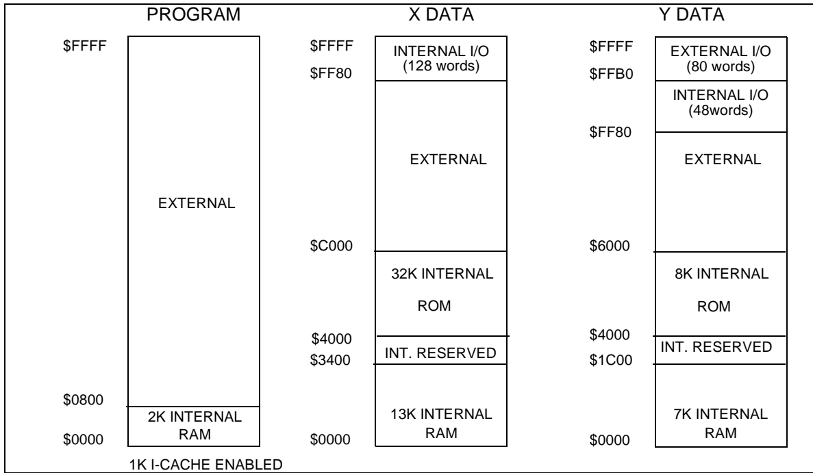
Figure 5-10 Memory Maps for MSW=(X,X), CE=1, MS=0, SC=1
