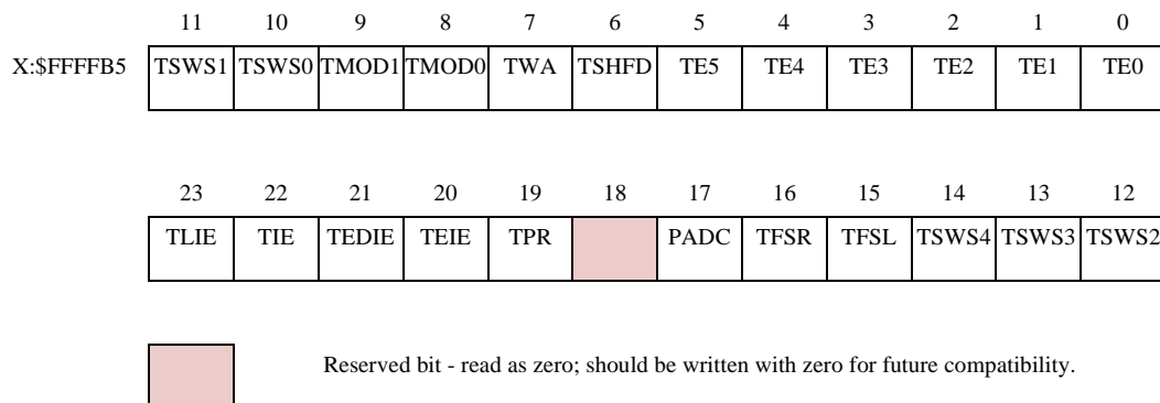
Figure 10-5 TCR Register
