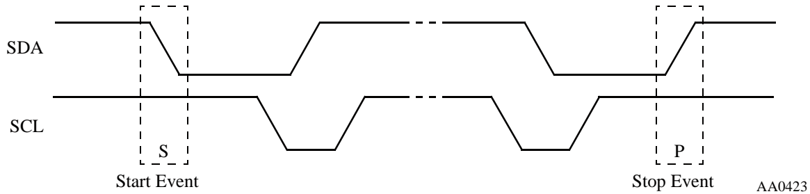
Figure 9-8 I 2 C Start and Stop Events
