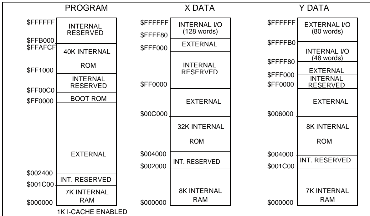
Figure 5-7 Memory Maps for MSW=(0,1), CE=1, MS=1, SC=0
