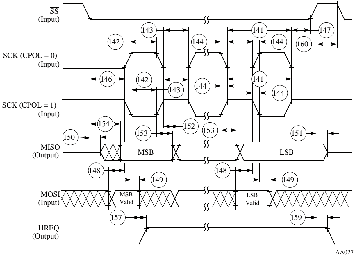
Figure 3-29 SPI Slave Timing (CPHA = 0)
