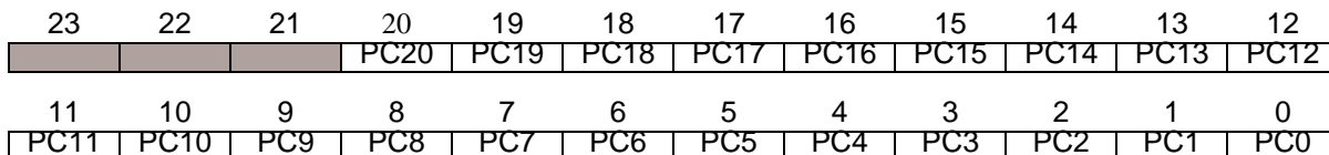
Figure 13-5 Timer Prescaler Count Register (TPCR)
