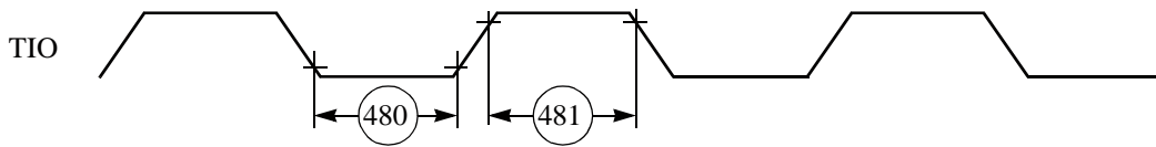
Figure 3-37 TIO Timer Event Input Restrictions
