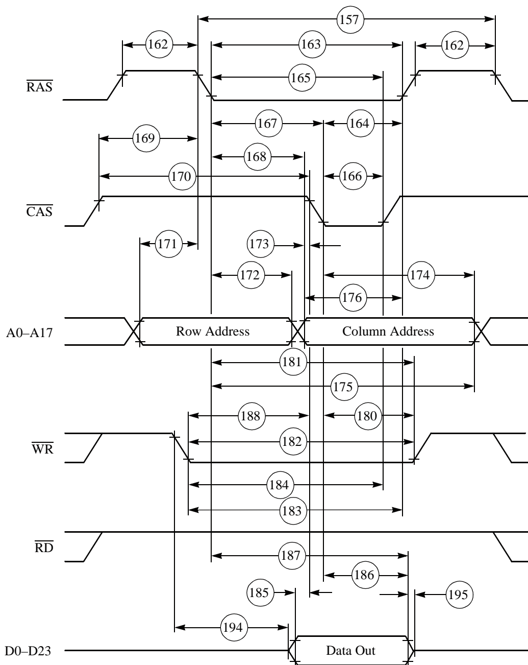
Figure 3-16 DRAM Out-of-Page Write Access
