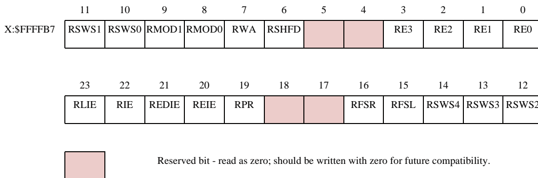
Figure 10-9 RCR Register
