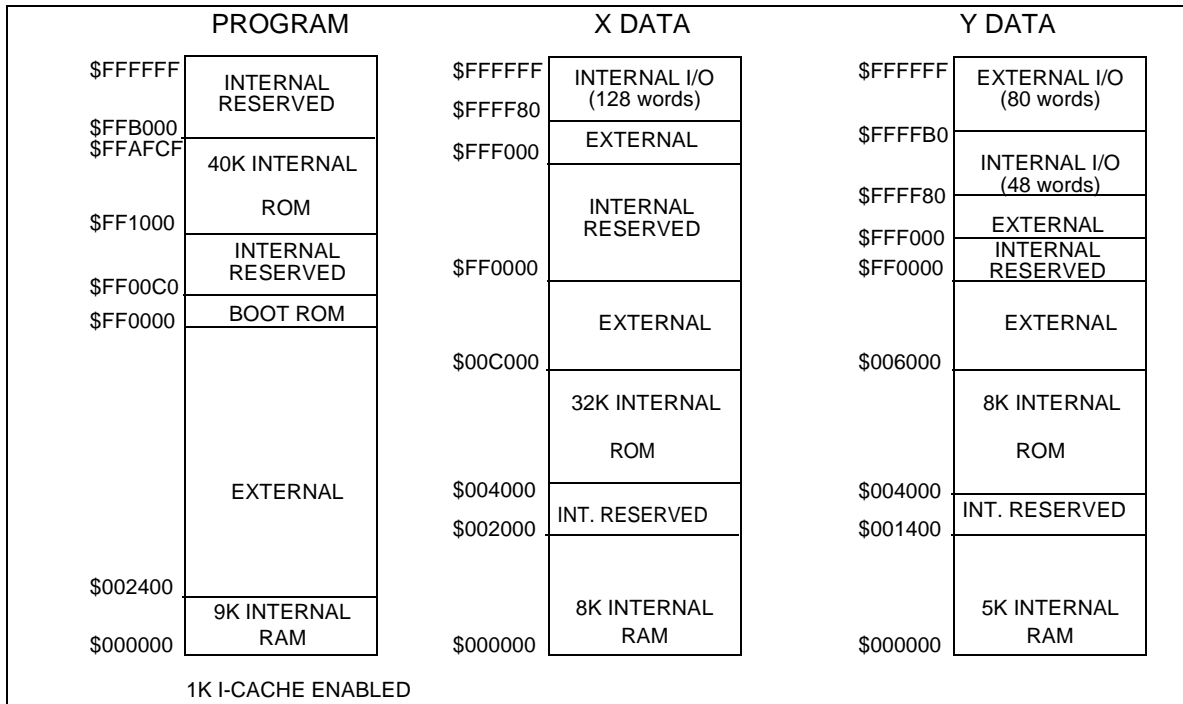
Figure 5-6 Memory Maps for MSW=(0,0), CE=1, MS=1, SC=0
