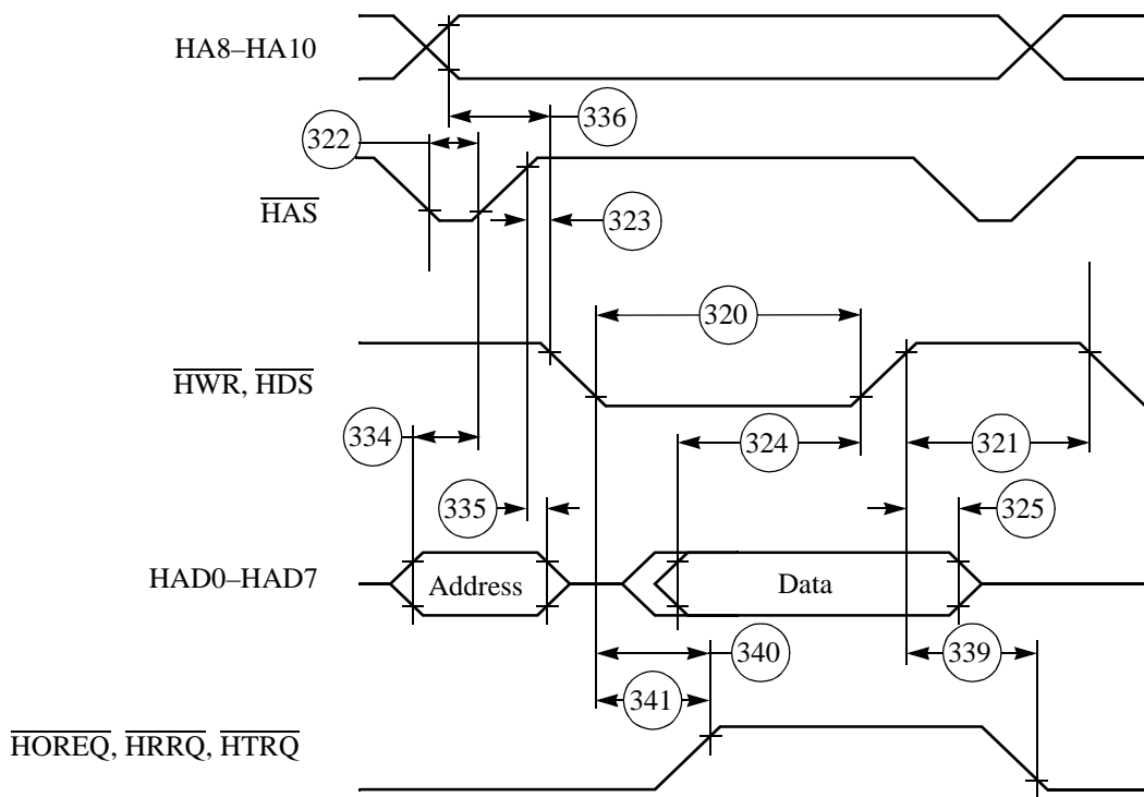
Figure 3-24 Write Timing Diagram, Multiplexed Bus
