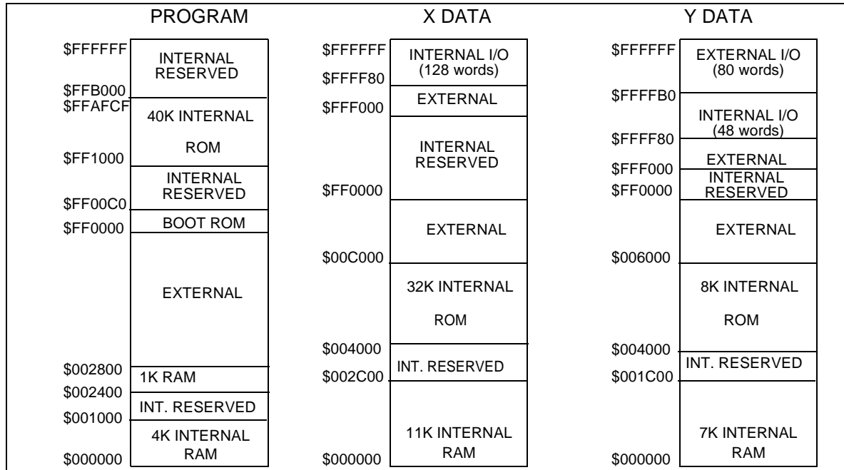
Figure 5-5 Memory Maps for MSW=(1,0), CE=0, MS=1, SC=0
