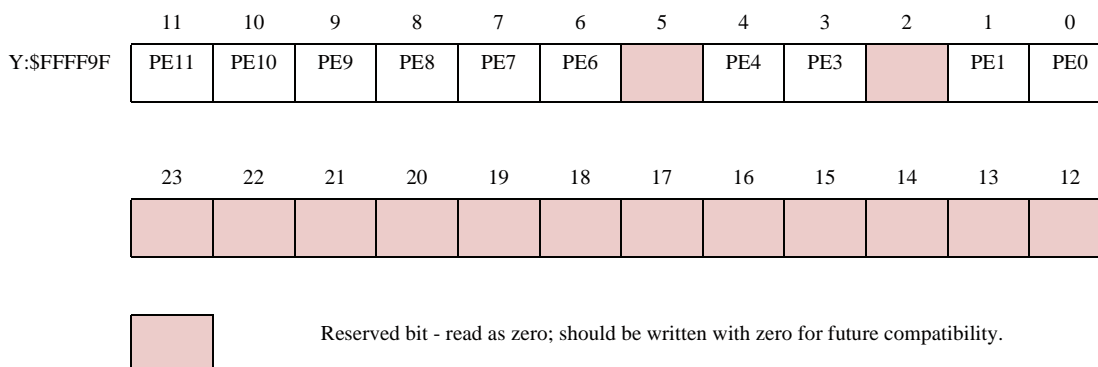
Figure 11-15 PCRE Register
