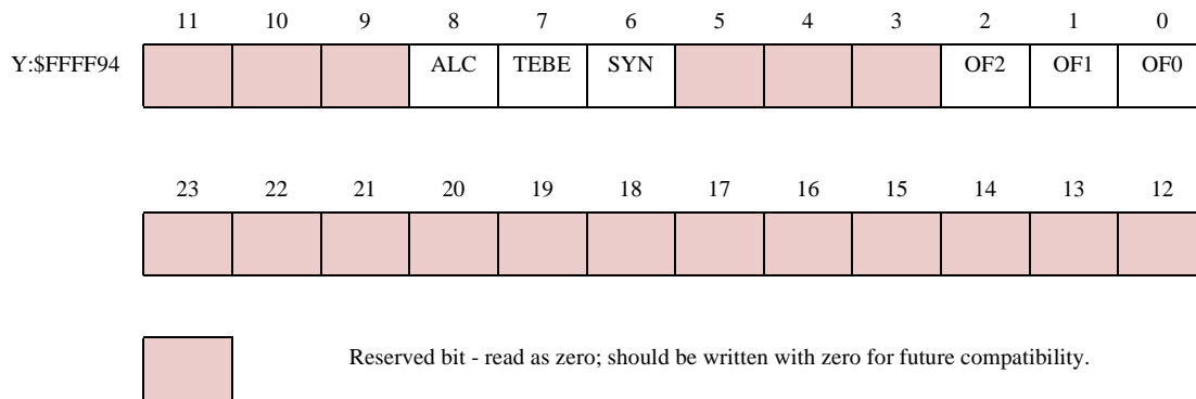
Figure 11-9 SAICR_1 Register
