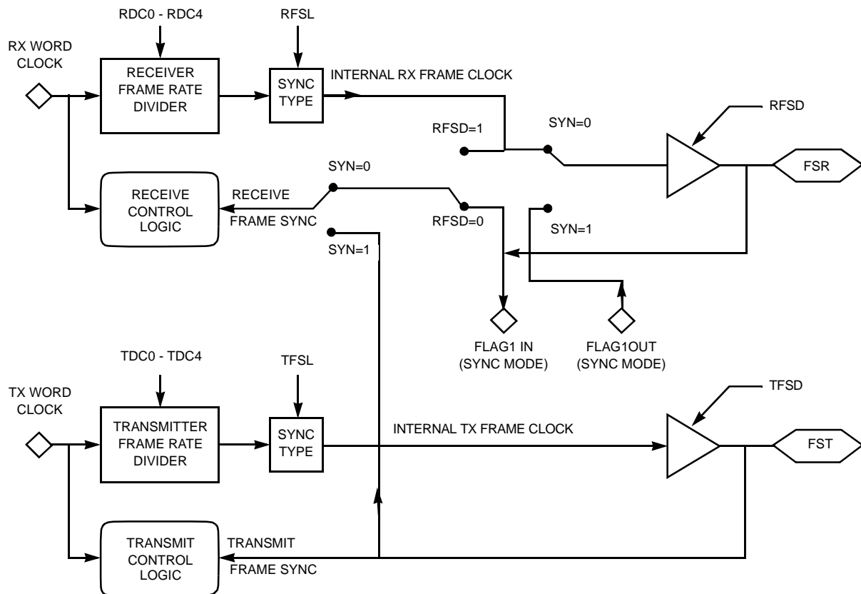
Figure 10-4 ESAI Frame Sync Generator Functional Block Diagram
