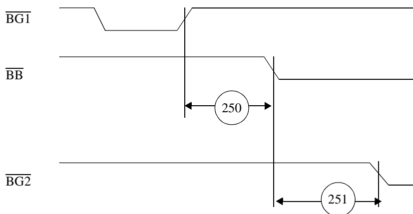
Figure 3-18 Asynchronous Bus Arbitration Timing
