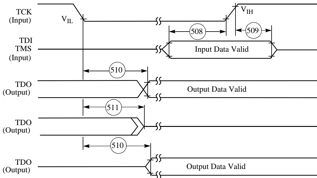
Figure 3-41 Test Access Port Timing Diagram
