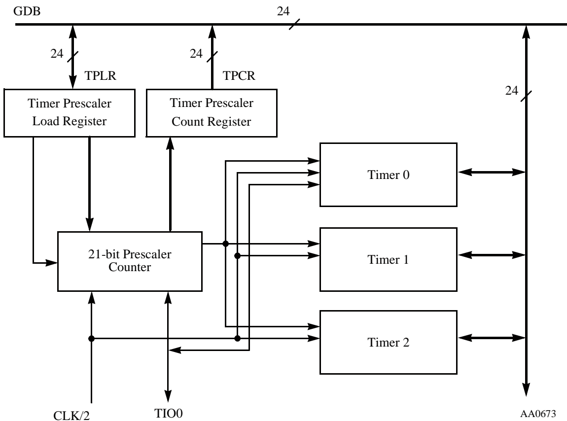
Figure 13-1 Timer/Event Counter Block Diagram
