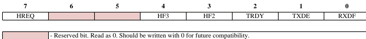
Figure 8-14 Interface Status Register (ISR)
