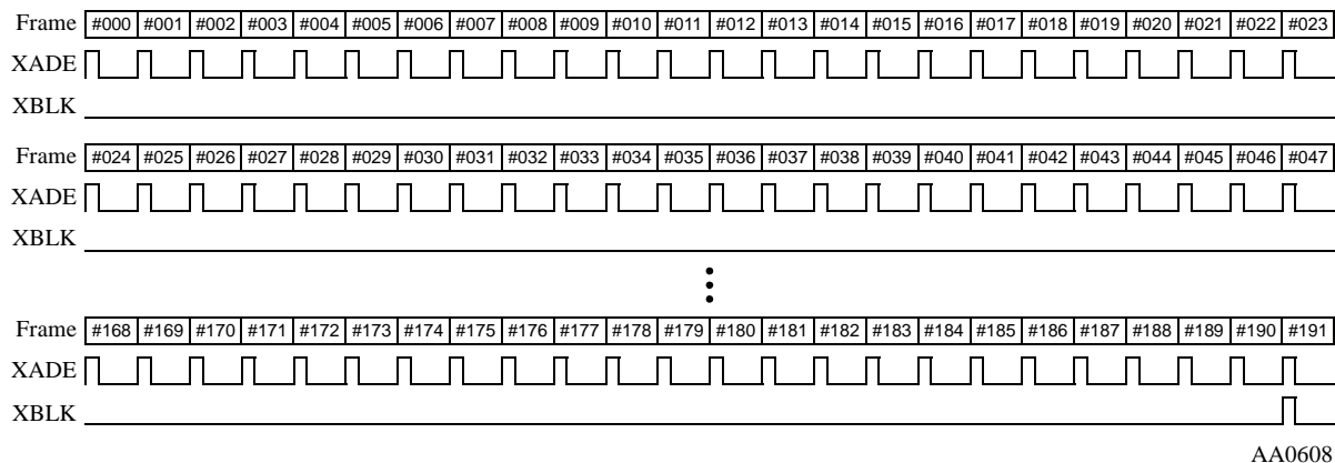
Figure 12-3 DAX Relative Timing
