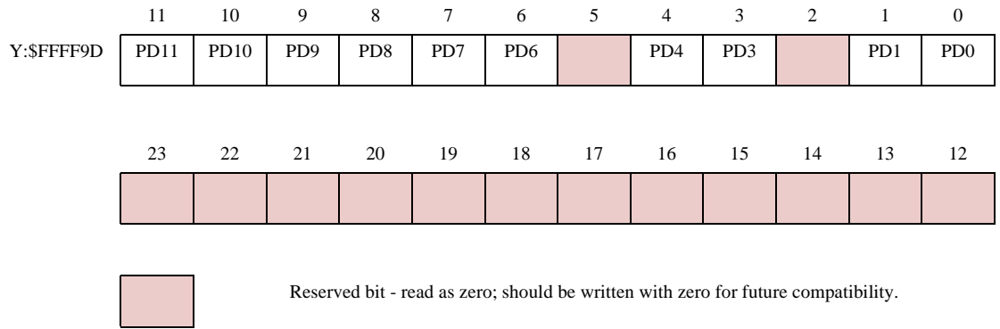
Figure 11-17 PDRE Register
