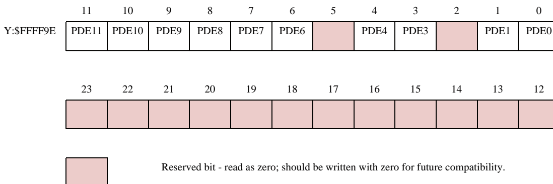
Figure 11-16 PRRE Register
