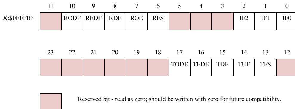
Figure 10-12 SAISR Register
