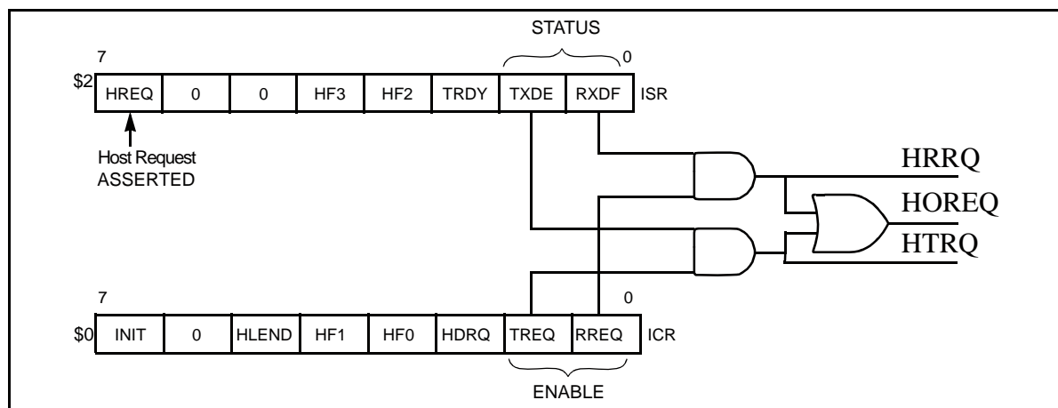
Figure 8-16 HDI08 Host Request Structure
