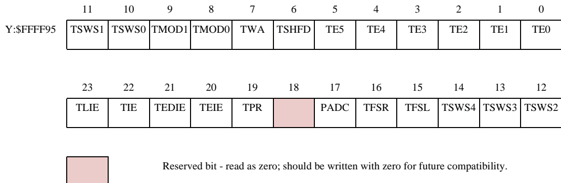
Figure 11-6 TCR_1 Register
