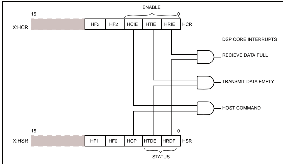
Figure 8-11 HSR-HCR Operation
