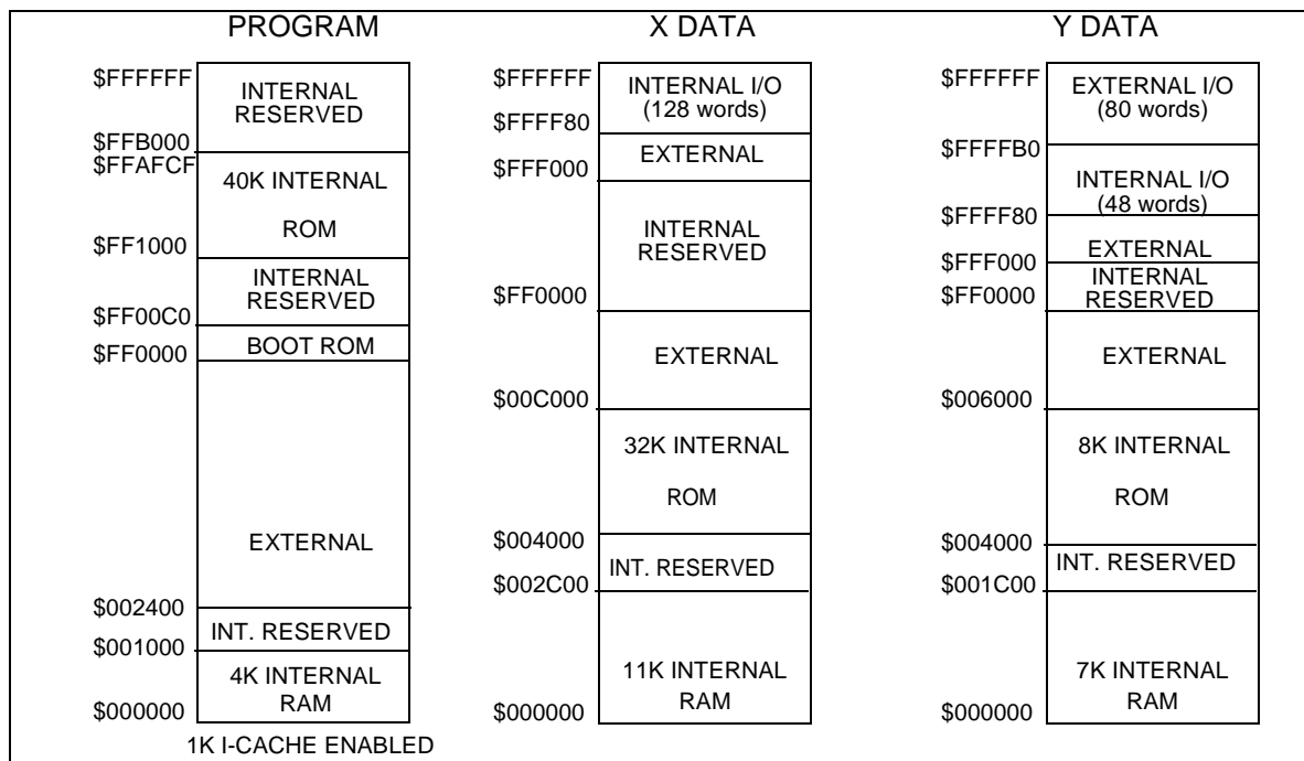
Figure 5-8 Memory Maps for MSW=(1,0), CE=1, MS=1, SC=0
