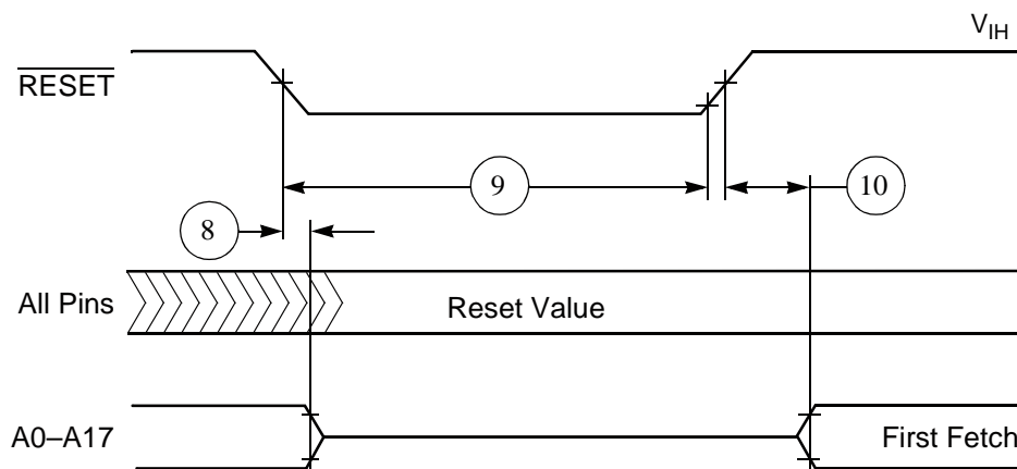
Figure 3-2 Reset Timing
