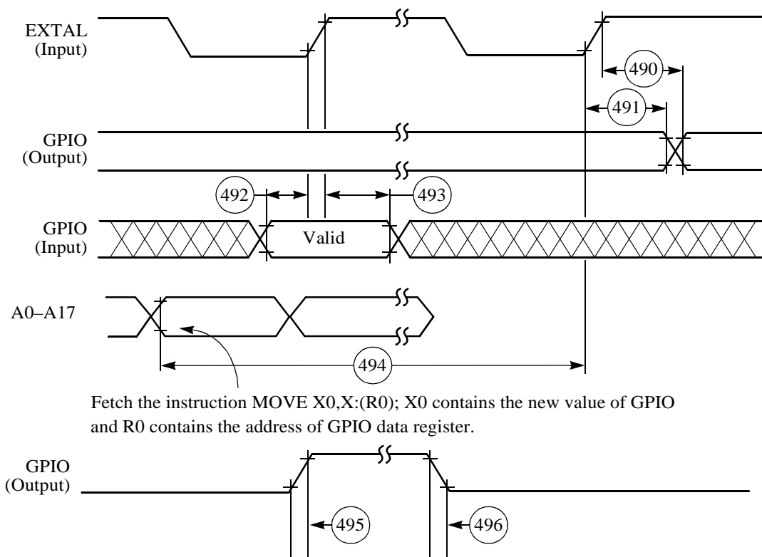
Figure 3-38 GPIO Timing
