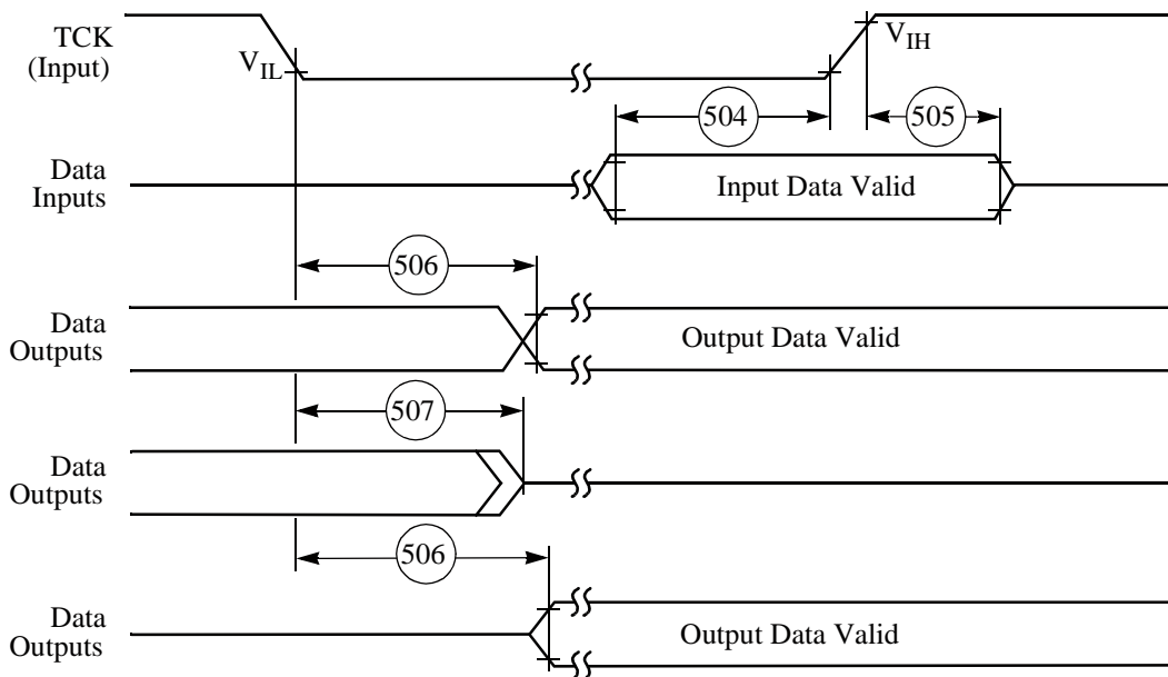
Figure 3-40 Boundary Scan (JTAG) Timing Diagram
