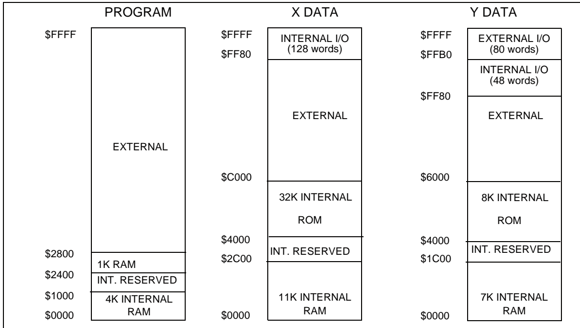
Figure 5-13 Memory Maps for MSW=(1,0), CE=0, MS=1, SC=1
