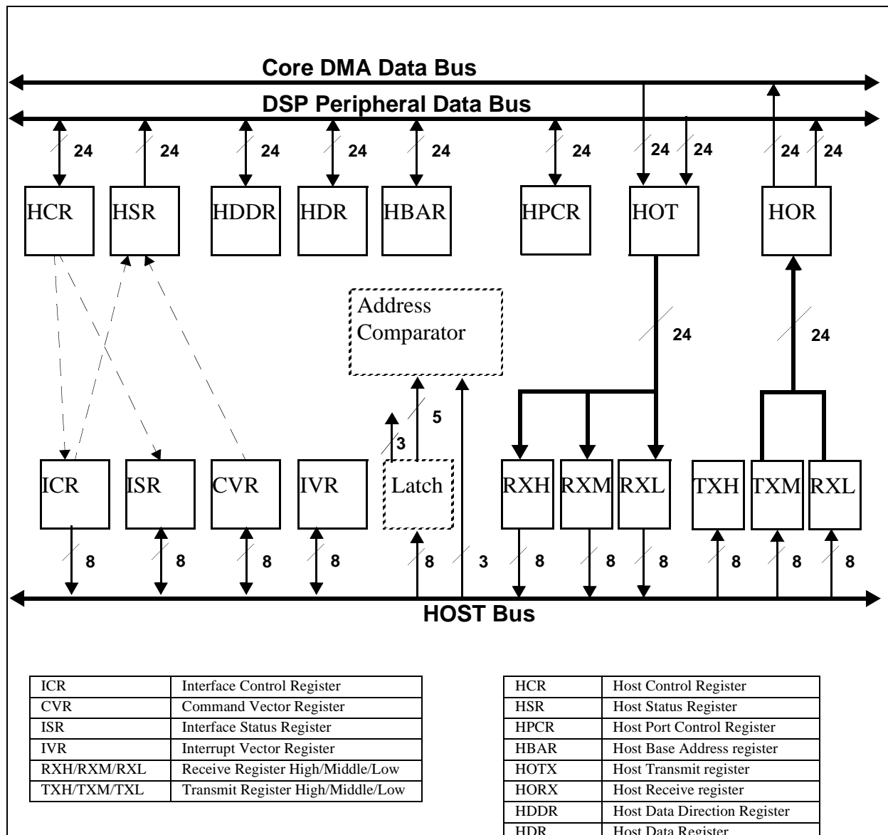
Figure 8-1 HDI08 Block Diagram
