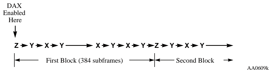
Figure 12-4 Preamble sequence
