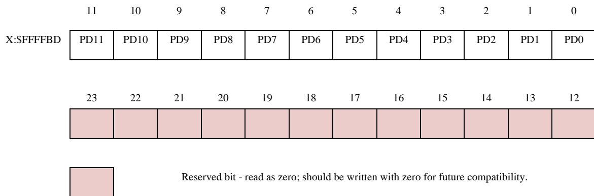
Figure 10-21 PDR Register
