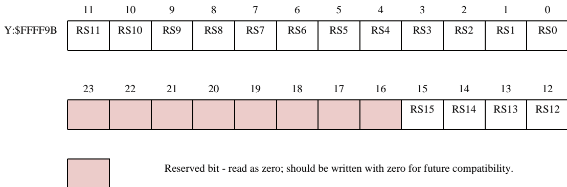
Figure 11-13 RSMA_1 Register
