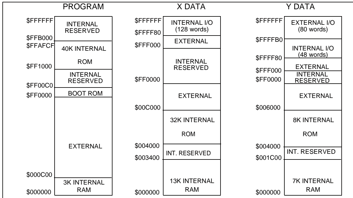
Figure 5-1 Memory Maps for MSW=(X,X), CE=0, MS=0, SC=0
