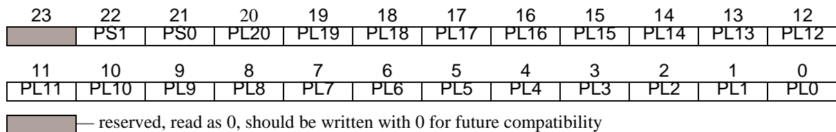
Figure 13-4 Timer Prescaler Load Register (TPLR)
