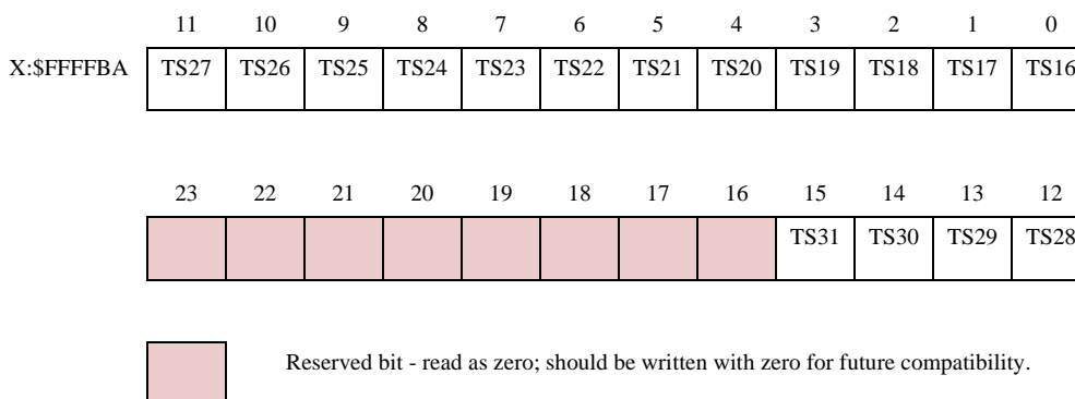
Figure 10-16 TSMB Register
