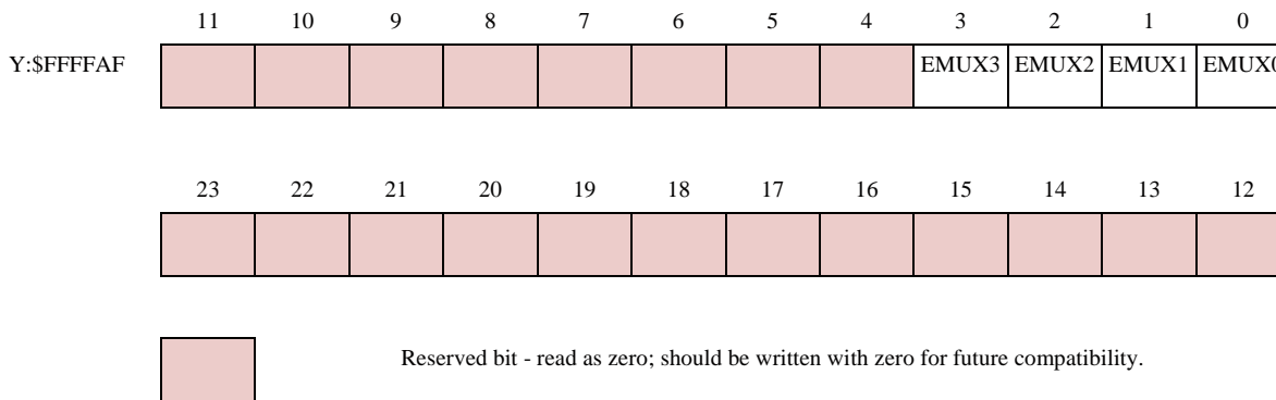
Figure 11-2 EMUXR Register
