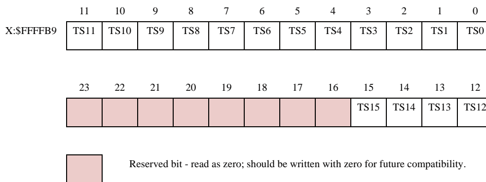
Figure 10-15 TSMA Register
