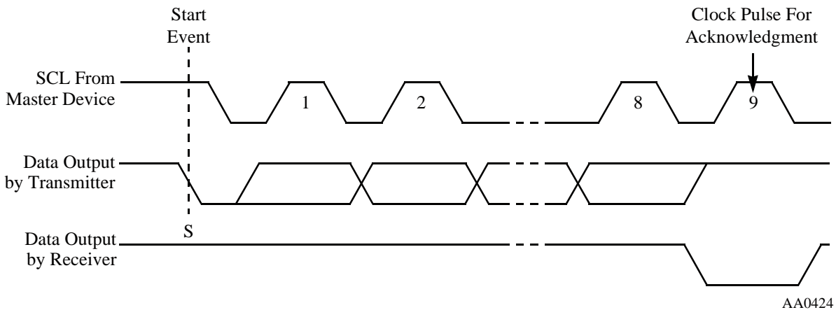
Figure 9-9 Acknowledgment on the I 2 C Bus
