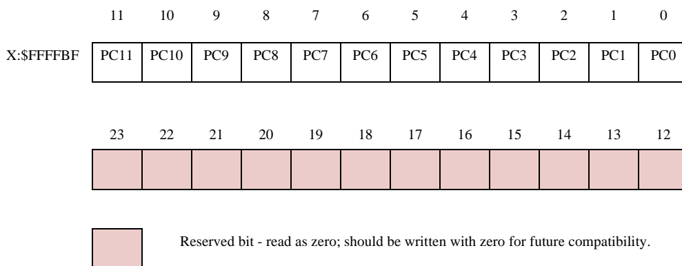
Figure 10-19 PCRC Register
