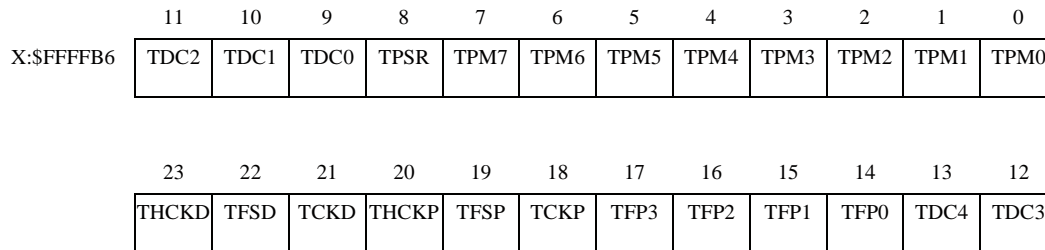
Figure 10-2 TCCR Register
