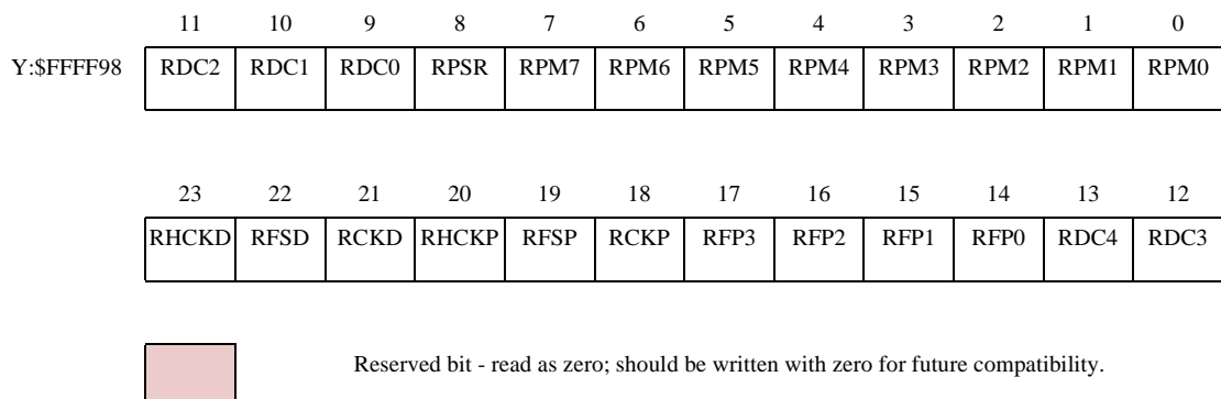
Figure 11-7 RCCR_1 Register
