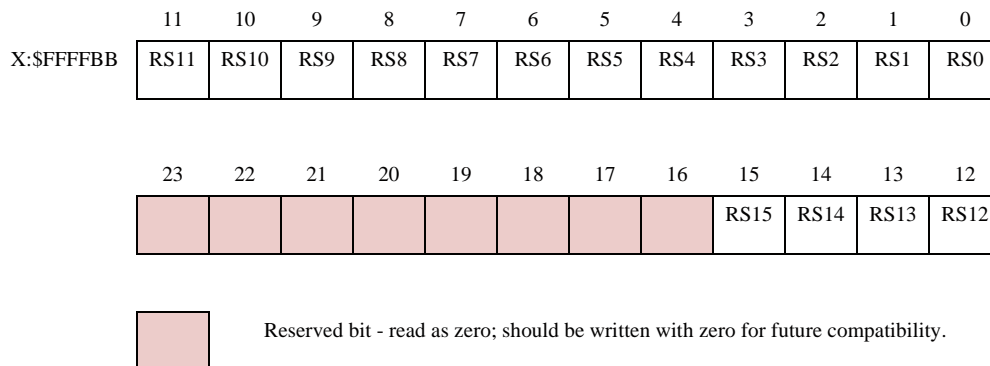
Figure 10-17 RSMA Register
