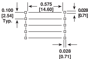
Footprint Diagram
