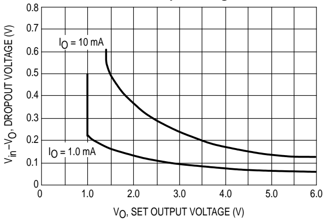
Figure 7. Dropout Voltage versus Set Output Voltage
