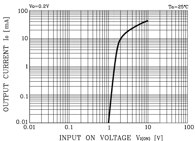
Fig. 1 I_o - V_{I(ON)}
