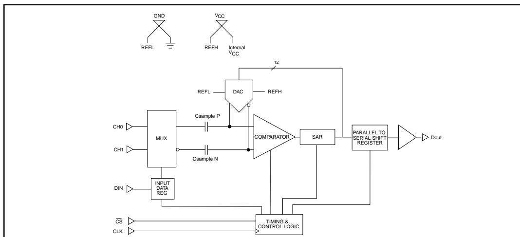
SP8538 Block Diagram
