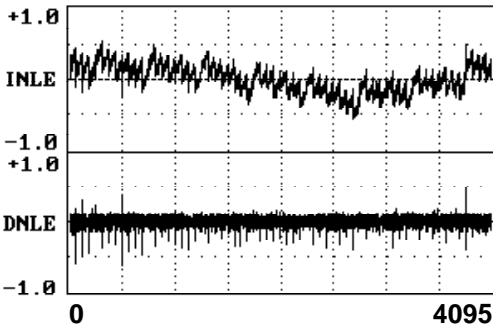
Vcc = 5.00V
