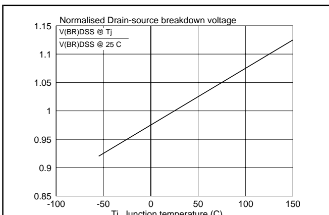
Fig.15. Normalised drain-source breakdown voltage. V_{(BR)DSS} / V_{(BR)DSS 25 C} = f(T_j)
