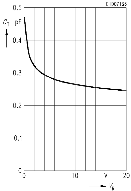
Diode capacitance C_T = f(V_R) f = 1 MHz.
