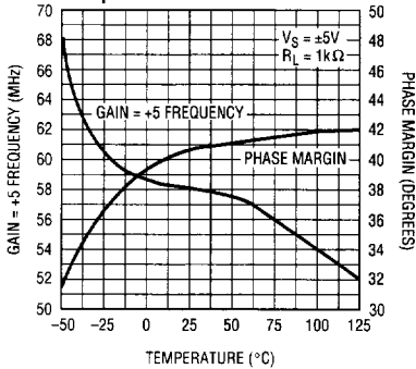
Gain and Phase Margin vs Temperature
