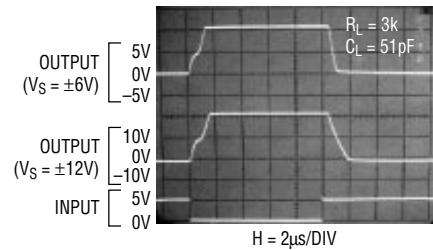
Output Waveforms
