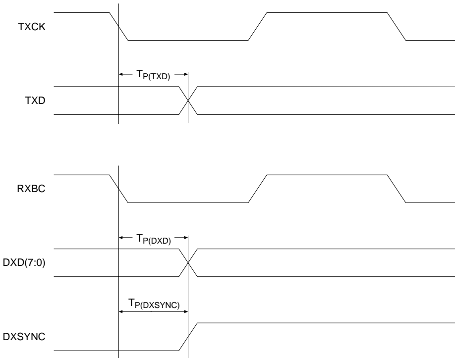
Figure 7. Output Timing
