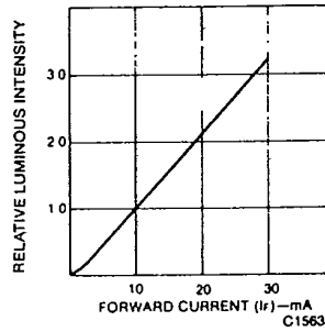
Fig. 2. Relative Luminous Intensity vs. Forward Current
