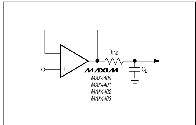
Figure 3. Capacitive-Load-Driving Circuit
