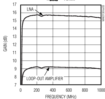
GAIN vs. FREQUENCY R BIAS = 10kΩ
