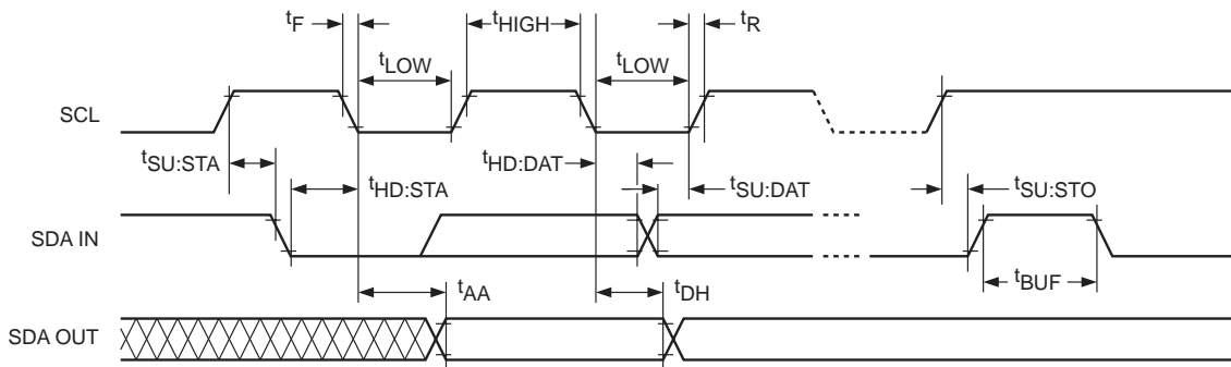
Figure 1. Bus Timing
